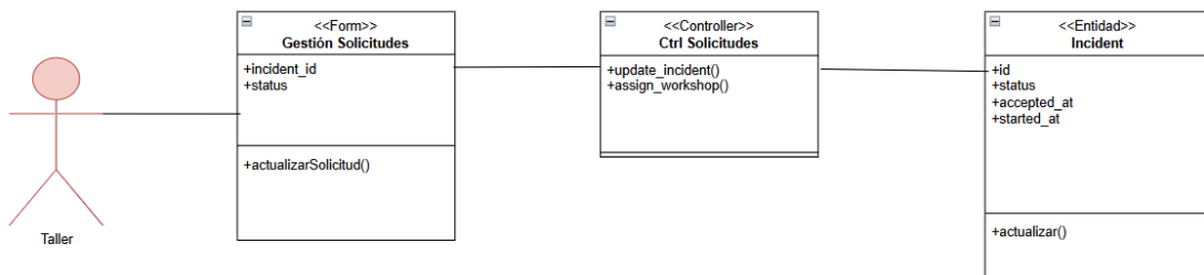
CU13- Gestionar Solicitudes
